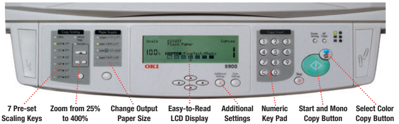
OKI® ES 3037 Family Scancopier Control Panel
